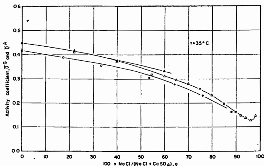
FIG. 10. Activity coefficients of \text{CaSO}_4 in the ternary system \text{CaSO}_4\text{--NaCl--H}_2\text{O} at 35^\circ\text{C} . Solid triangles, activity coefficients in gypsum-saturated solutions ( \gamma^G ), calculated using the Robinson-Stokes extension of the Debye-Hückel formula; open triangles, \gamma^G calculated from the observed \text{CaSO}_4 solubilities in the ternary system; open circles, activity coefficients in anhydrite-saturated solutions ( \gamma^A ), calculated using the Robinson-Stokes extension of the Debye-Hückel formula and the 'consistent' thermochemical data for the system \text{CaSO}_4\text{--H}_2\text{O} ; solid circles, \gamma^A calculated by extrapolating the \gamma^A/\gamma^G ratio derived from the Debye-Hückel formula, as explained in the text. The reversal of slope at the high NaCl end indicates the 'salting-out' effect on gypsum in NaCl-rich solutions.
