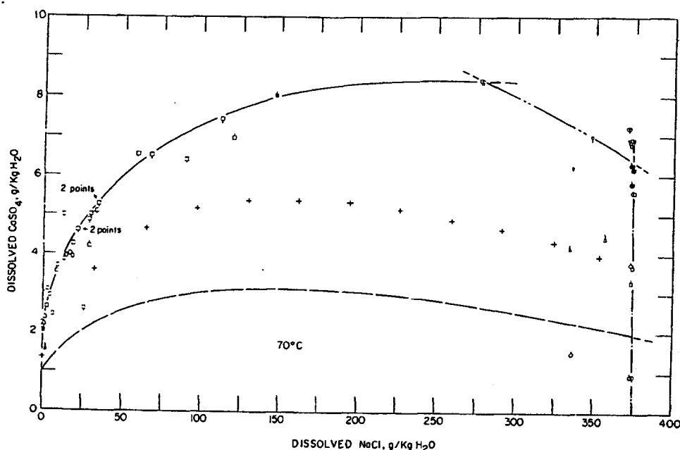
FIG. 6. Solubility at 70° C. See caption for Fig. 5 for explanations. Dash-dot-dot line, bassanite solubility.
